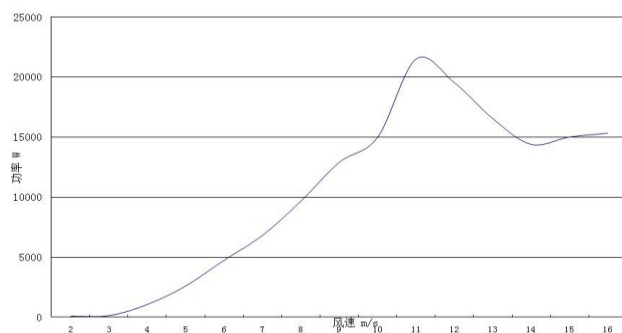
EN-20KW-E wind turbine power curve
