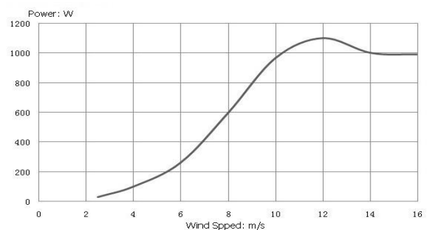
EN-1KW-L wind turbine power curve
